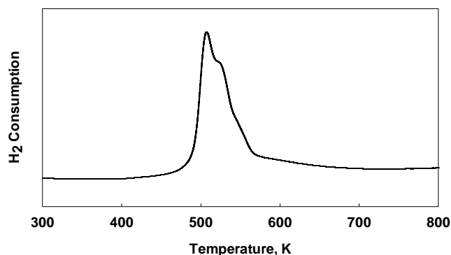
Fig. 2 TPR profile of Cu-ZnO/Al 2 O 3 catalysts
