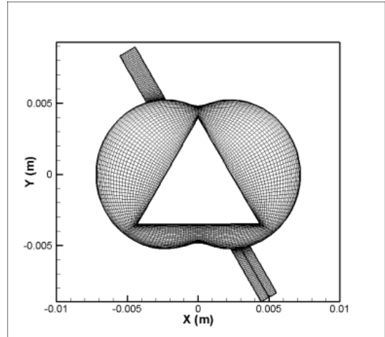
Fig. 7 The grid layout of case Geo-3
