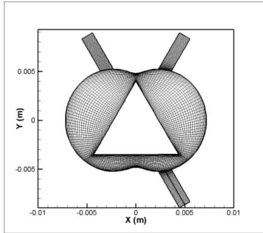
Fig. 9 The grid layout of case Geo-4
