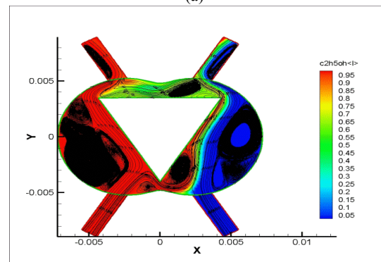
Fig. 12 The alcohol concentration contours and streamline of case Geo-5 (a)Re=10 \omega = 150 r.p.m. (b)Re=300 \omega = 30 r.p.m.
