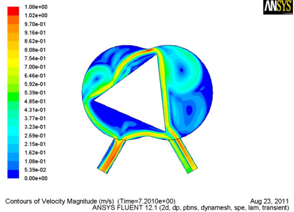
(a) Re=10 \omega = 150 r.p.m. (b) Re=300 \omega = 30 r.p.m.
