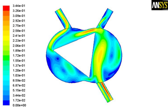
Contours of Velocity Magnitude (m/s) (Time=1.5200e-01) Jul 11, 2011 ANSYS FLUENT 12.1 (2d, dp, pbns, dynamesh, spe, lam, transient)
