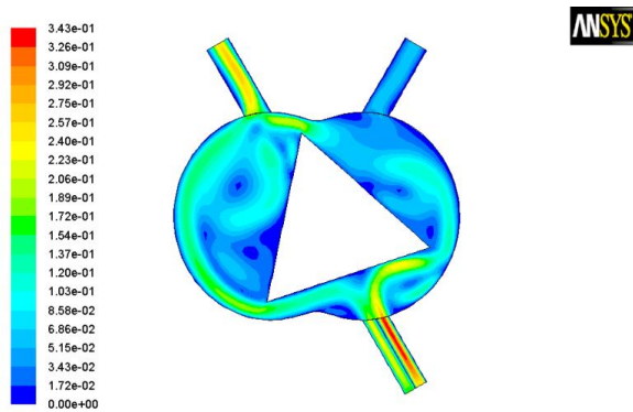
Contours of Velocity Magnitude (m/s) (Time=8.1010e+00) Jul 11, 2011 ANSYS FLUENT 12.1 (2d, dp, pbns, dynamesh, spe, lam, transient)
