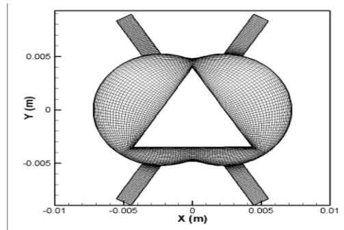
Fig. 11 The grid layout of case Geo-5
