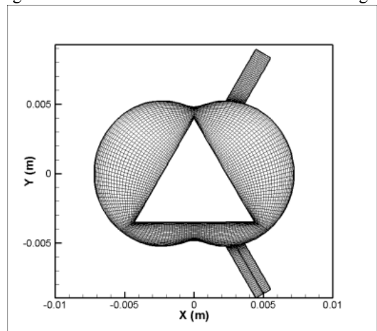
Fig. 5 The grid layout of case Geo-2
