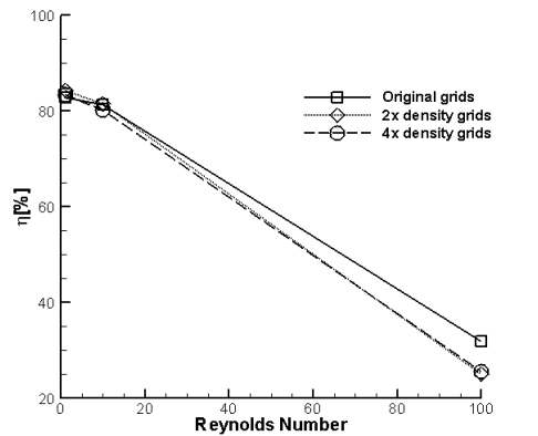
Fig. 3 The grids refinement test results
