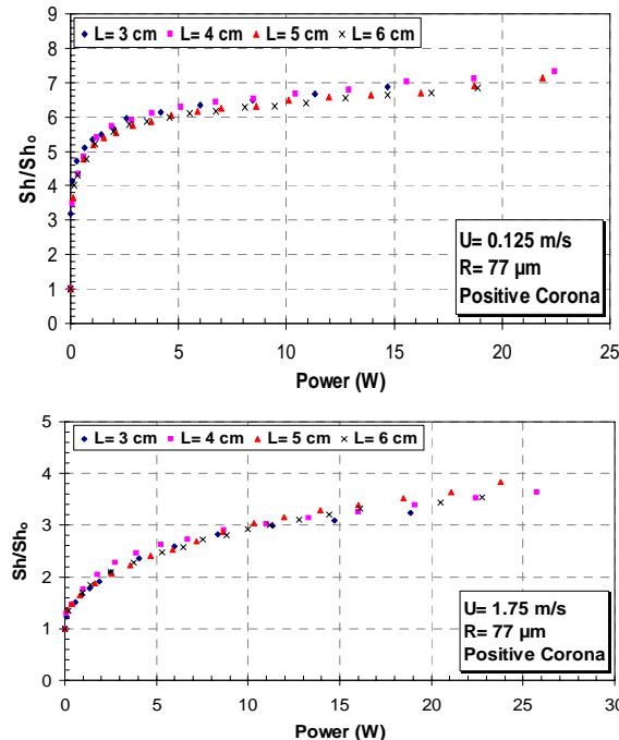
Fig. 6 Evaporation enhancement versus electrical power
