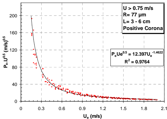
Fig. 8 EHD performance versus corona wind velocity
