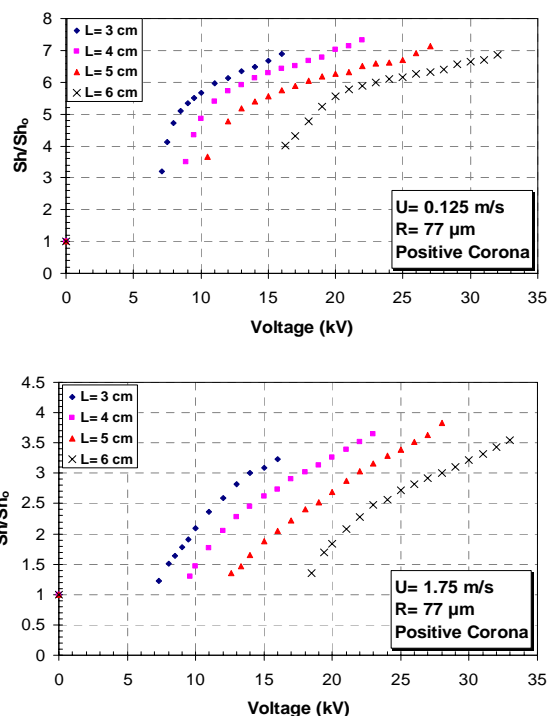
Fig. 2 Evaporation enhancement versus voltage
