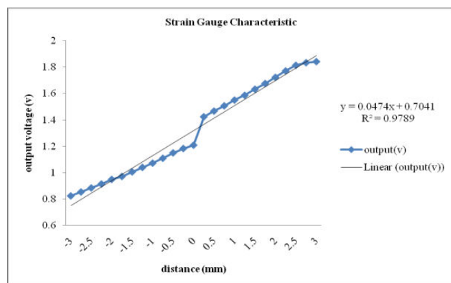
Fig. 2 The strain gauge characteristic
