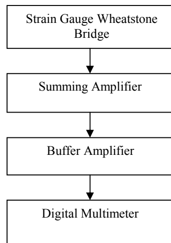
Fig. 1 The block diagram of the measurement system
