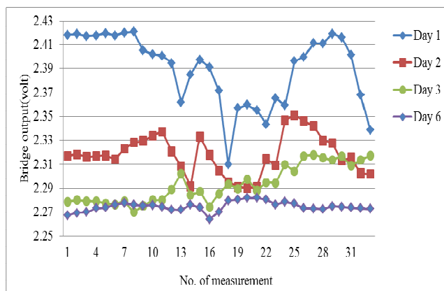
Fig. 6 Comparisons of stem variations for the 6 days
