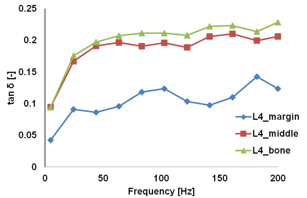
Fig. 7 Damping of all tested positions of the endplate couched in relation of \tan \delta and frequency.
