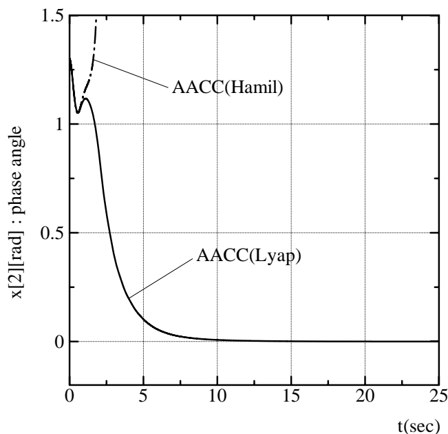
Fig.11 Responses of AACC(Hamil), AACC(Lyap) (x^T(0) = [0, 1.3, 0])
