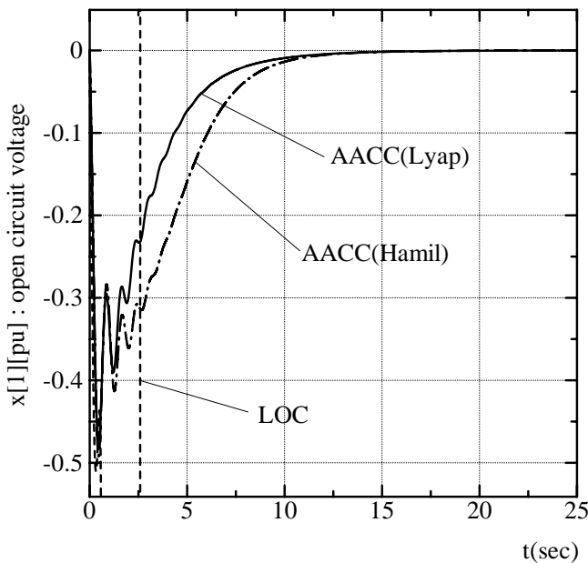
Fig. 4 Responses of LOC, AACC(Hamil), AACC(Lyap) ( x^T(0) = [0, 1.2, 0] )
