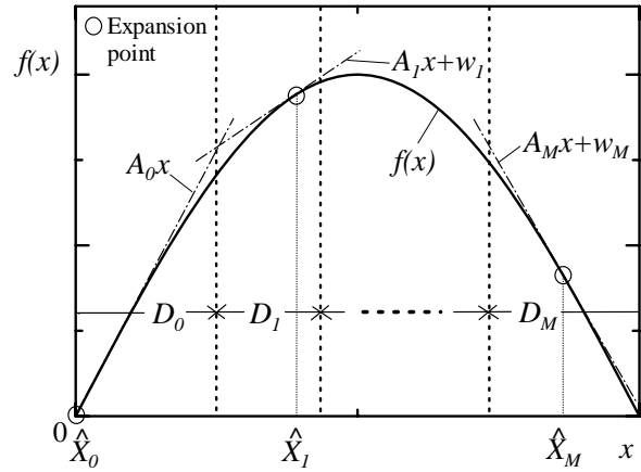
Fig. 1 Sectionwise linearization
