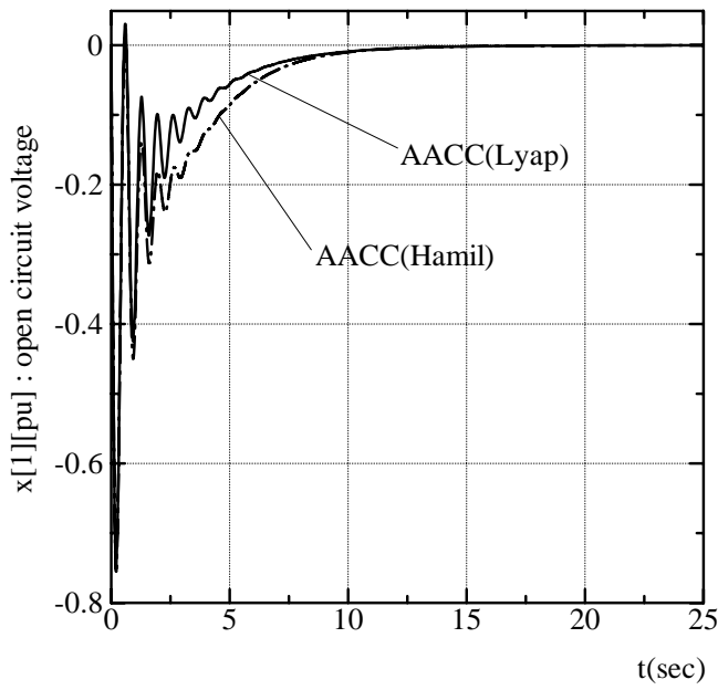
Fig. 7 Responses of AACC(Hamil), AACC(Lyap) (x^T(0) = [0, 1.0, -5])
