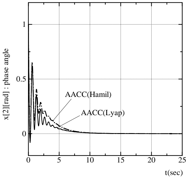
Fig. 8 Responses of AACC(Hamil), AACC(Lyap) (x^T(0) = [0, 1.0, -5])
