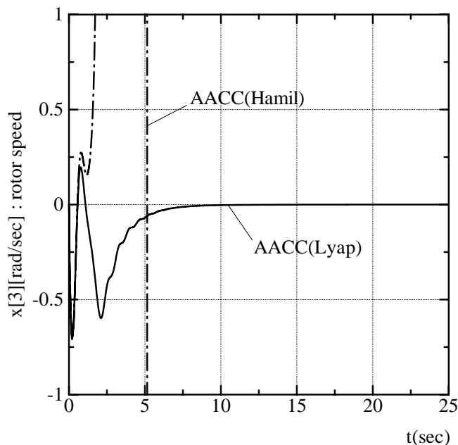
Fig.12 Responses of AACC(Hamil), AACC(Lyap) (x^T(0) = [0, 1.3, 0])
