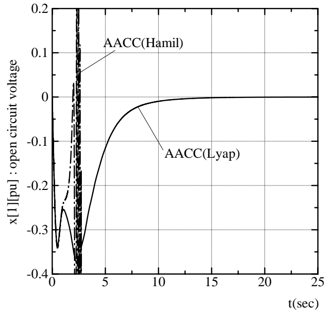
Fig.10 Responses of AACC(Hamil), AACC(Lyap) (x^T(0) = [0, 1.3, 0])
