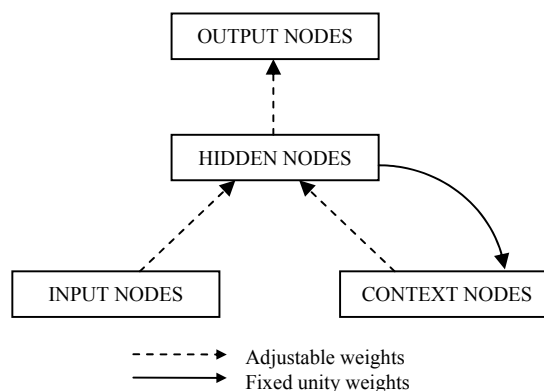
Fig. 1 Architecture of the Elman network
