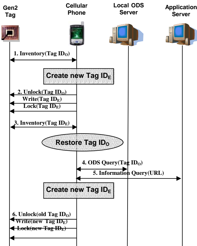
Fig. 3 Procedure of hiding Original Tag ID
