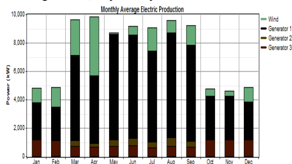
Fig. 3 Monthly average electric production
