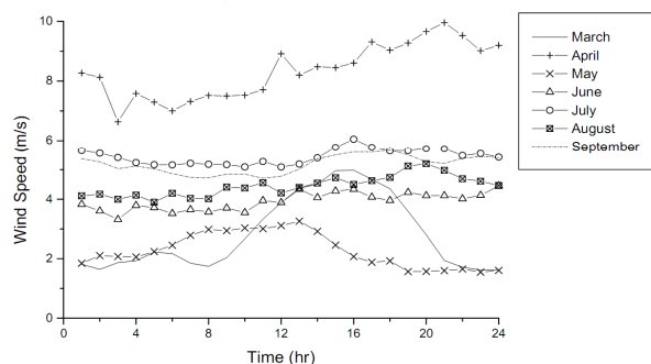
Fig. 1 Average wind speed at Sandwip in March–September
