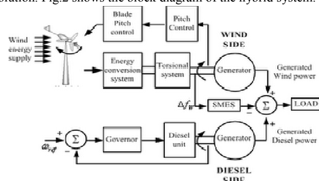
Fig. 2 Block diagram of wind-diesel hybrid power system
