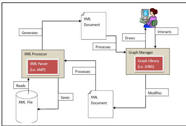
Fig. 6 The architecture of VIC
