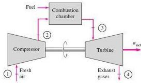
Fig. 1. Simple cycle gas turbine
