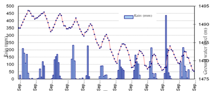
Fig. 1 The rainfall(mm) and groundwater hydrograph(m) of Kavarmaharlool plain
