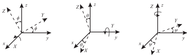
Fig. 2. Attitude definition
