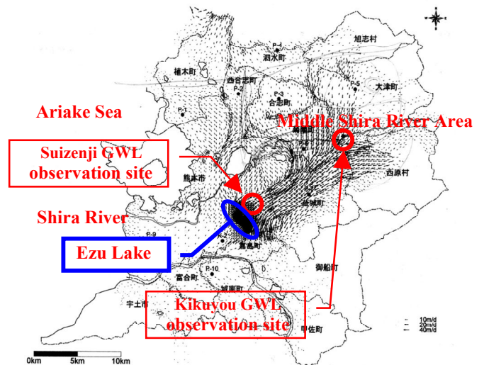
Fig. 6 Groundwater flow in second aquifer in Kumamoto Groundwater Basin (Oct., 2004) [1]
