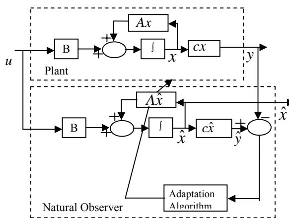
Fig. 1 Natural observer with adaptation
