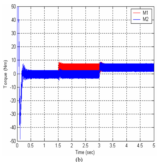
Fig. 7 Unbalanced load test Kubota's method
