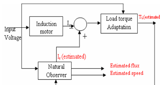
Fig. 2 Block diagram representation
