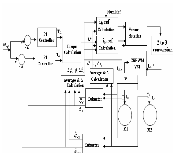
Fig 4 Configuration of parallel connected induction motor
