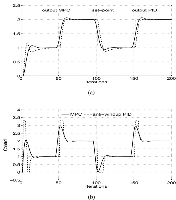
Fig. 4. Closed-loop simulation results for 1st order system
