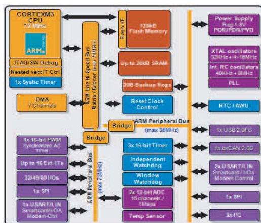
Fig. 1. STM32F103RB block diagram
