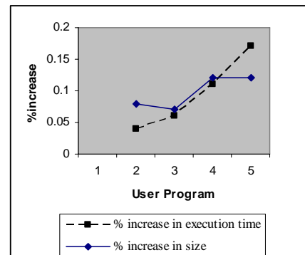
Fig. 5 Percentage increase in execution time and size of user program
