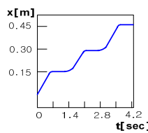
(a) ZMP trajectory in sagittal plane
