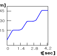
(b) ZMP trajectory in lateral plane
