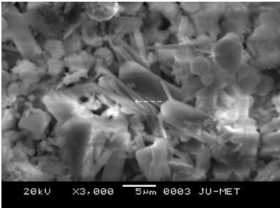
Fig. 9 SEM image of geopolymer mortar with 6.5% Na 2 O and EDAX spectrum at the arrow point after 12 weeks in 10% sulphuric acid
