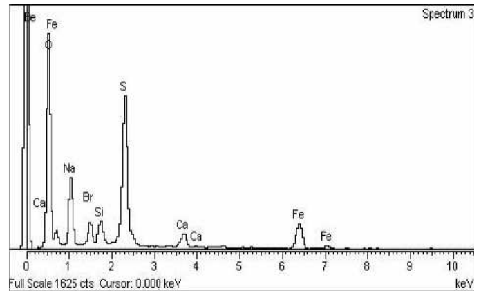
Fig. 9 SEM image of geopolymer mortar with 6.5% Na 2 O and EDAX spectrum at the arrow point after 12 weeks in 10% sulphuric acid
