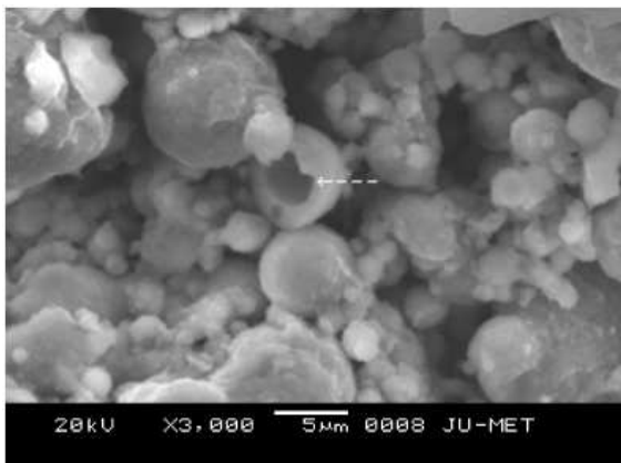
Fig. 6 SEM image of geopolymer mortar with 5% Na 2 O and EDAX spectrum at the arrow point before exposure
