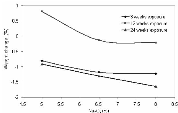
Fig. 4 Variation of weight with % Na 2 O
