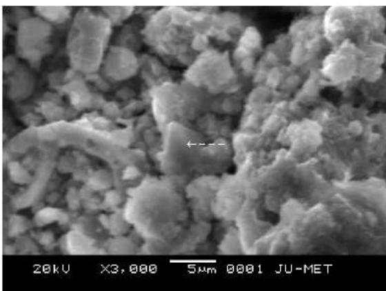
Fig. 7 SEM image of geopolymer mortar with 6.5% Na 2 O and EDAX spectrum at the arrow point before exposure
