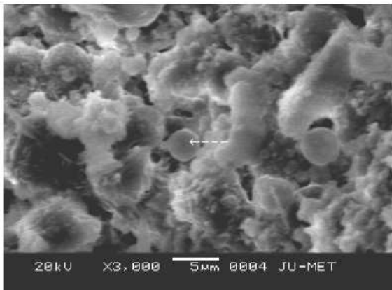
Fig. 8 SEM image of geopolymer mortar with 5% Na 2 O and EDAX spectrum at the arrow point after 12 weeks in 10% sulphuric acid
