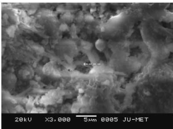
Fig. 10 SEM image of geopolymer mortar with 8% Na 2 O and EDAX spectrum at the arrow point after 12 weeks in 10% sulphuric acid
