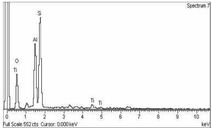
Fig. 6 SEM image of geopolymer mortar with 5% Na 2 O and EDAX spectrum at the arrow point before exposure
