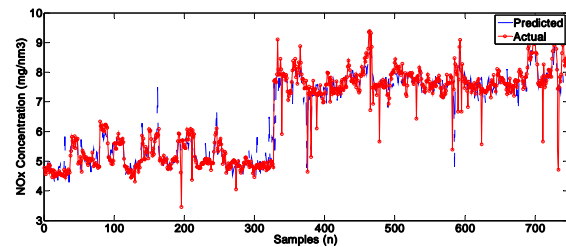
Fig. 3 NO x training data for BPNN
