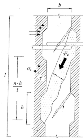
Fig. 2 Model for the shear transfer [2]
