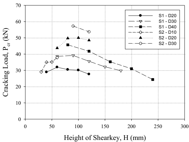
Fig. 8 Minimum cracking load ( \beta = 30^\circ , S = 20 mm)
