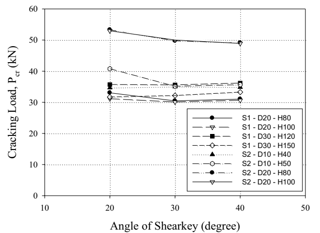
Fig. 11 Cracking load with tooth angle ( S = 20 mm)
