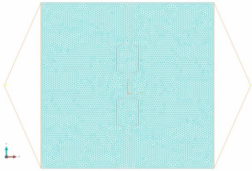
Fig. 4 Finite element model for shear key
