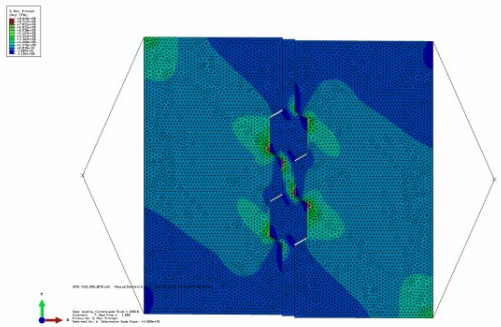
Fig. 5 Contour of maximum principal stress
