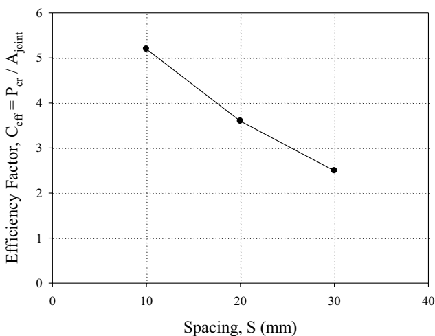
Fig. 13 Efficiency factor with spacing (N = 2, D = 20 mm, H = 80 mm, β = 30°)
