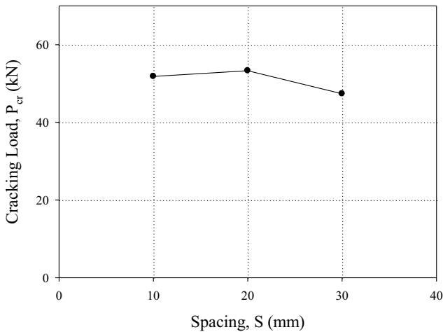
Fig. 12 Cracking load with spacing (N = 2, D = 20 mm, H = 80 mm, β = 30°)
