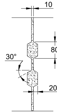
Fig. 14 Dimensions of longitudinal joint for the precast slab modular bridge (span length is 10 m)
