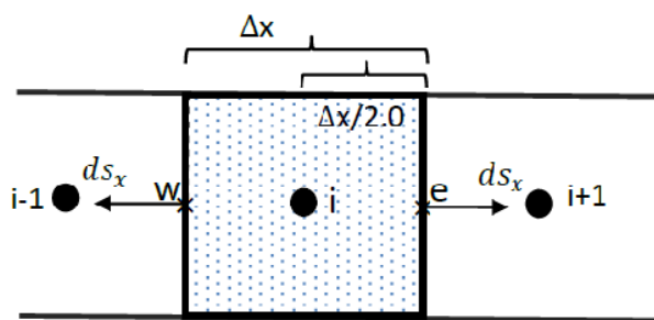
Fig. 1 Ordinary Control Volume
