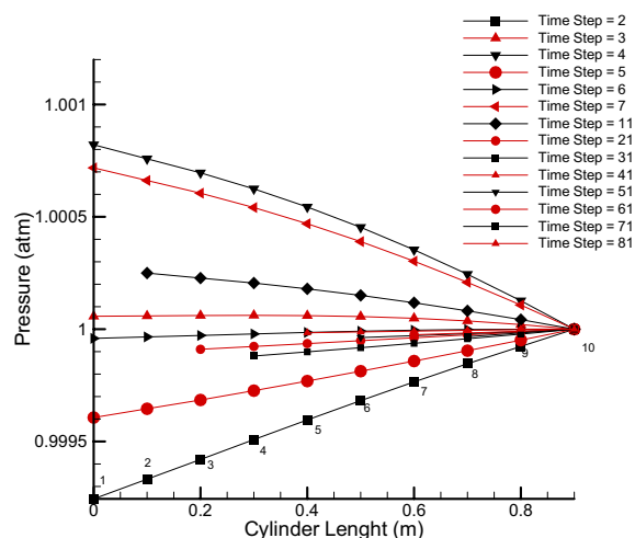
Fig. 10 Pressure distribution along the cylinder at different time steps calculated by the Image Point method
