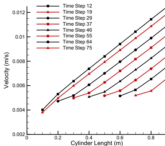
Fig. 11 Velocity of Nodes for several time steps via our proposed method
