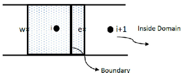
Fig. 2 Ghost Control Volume type one
