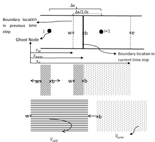
Fig. 5 Ghost Control Volume Type One
