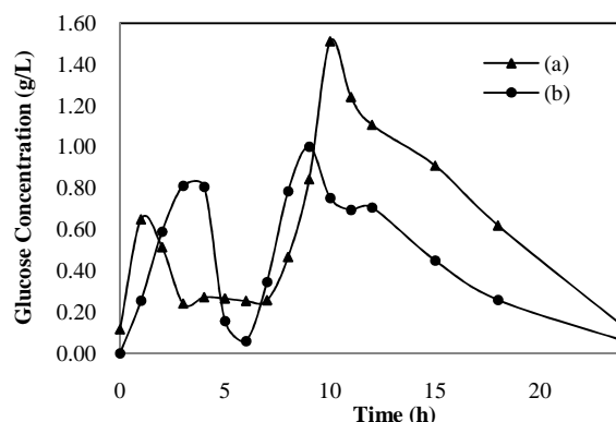
Fig. 1 Effects of particle size for 60 mesh (a) and 40 mesh (b) of casava residue on the glucose concentration produced from the hydrolysis of casava residue at 37 °C using the bacterial strain A 002.
