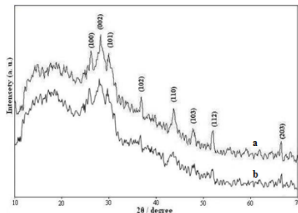
Fig. 2 High-angle XRD pattern of (a) sample II (b) sample I.
