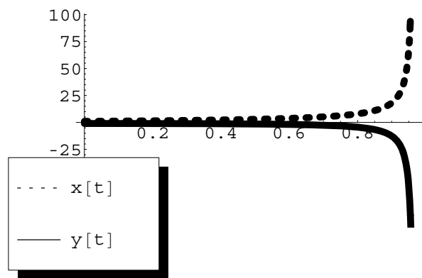
Fig. 2. Blow up in the Volterra-Lotka model
