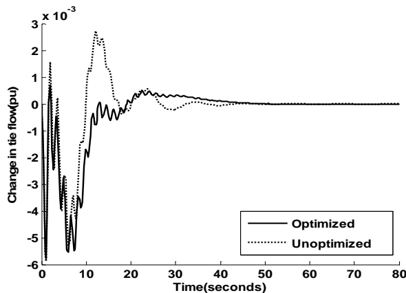
Fig. 15 change in tie line power flow
