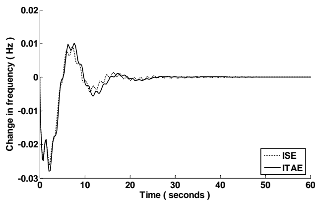
Fig. 4 frequency change in thermal area (using GA)
