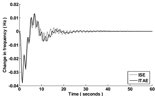
Fig. 5 frequency change in hydro area (using GA)
