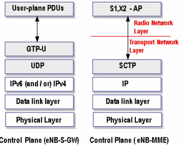
Fig. 3 (S1 and X2) Interface User and Control Planes
