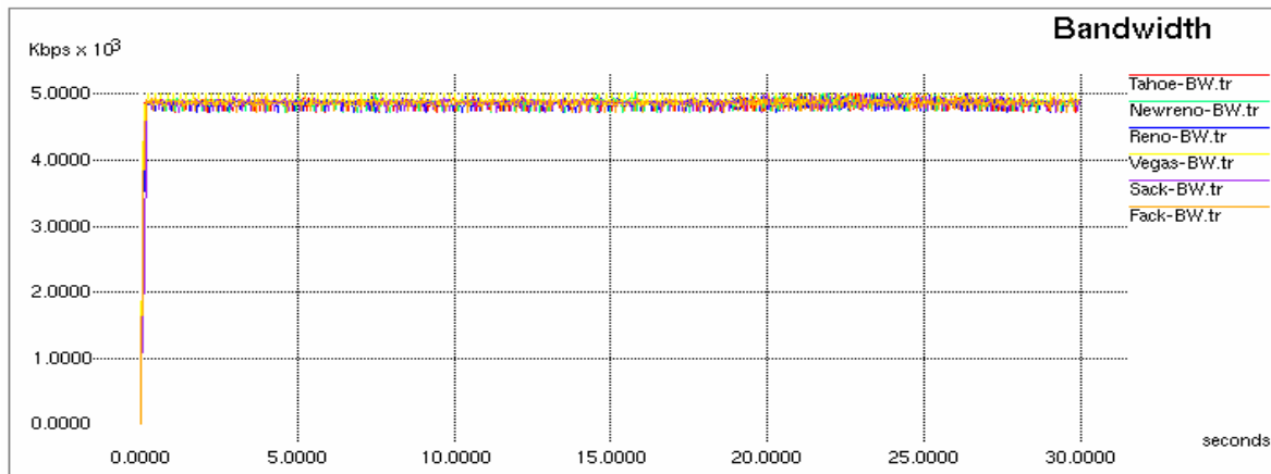
Fig. 8 Comparison Bandwidths versus time of Different TCP variants
