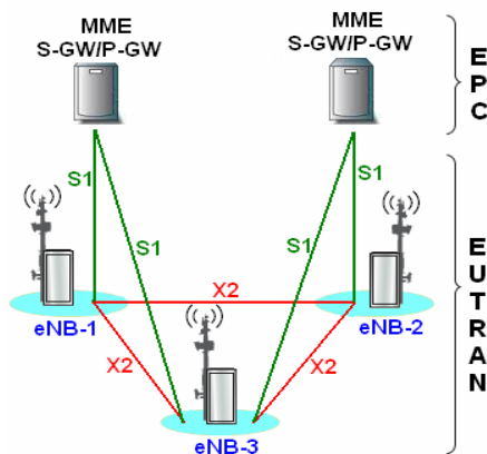
Fig. 2 E-UTRAN and EPC Architecture
