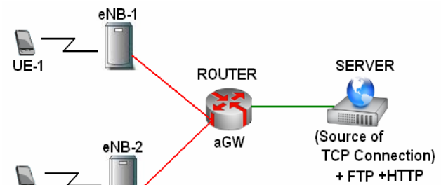
Fig. 4 Proposed Topology
