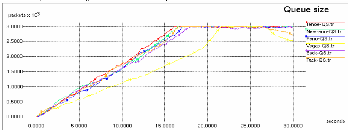
Fig. 6 Comparison Queue sizes versus time of different TCP variants
