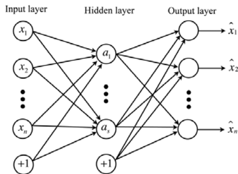
Fig. 2. An autoencoder feature extractor
