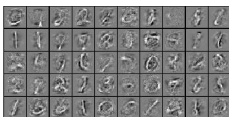
Fig. 9. Visualization samples of learned bases of 50 hidden neurons from MNIST handwritten digit
