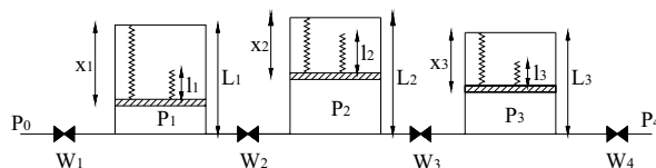
Fig. 1 Three-tank system
