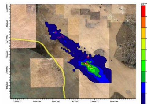
Fig. 7b Isoleths plot for the maximum daily average ground level concentrations of non-methane hydrocarbons in \mu\text{g}/\text{m}^3
