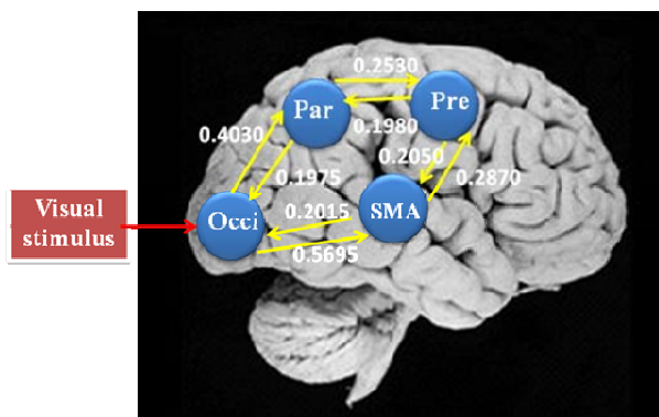
Fig. 5 The best model with the visual stimulus
