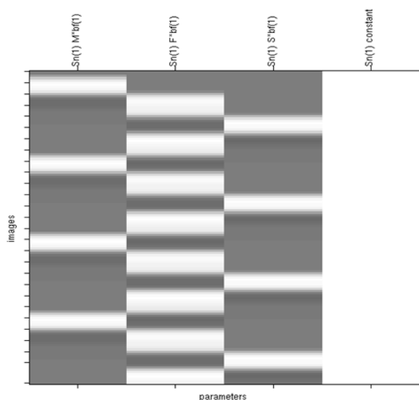
Fig. 1 SPM's design matrix of the stimulus sequence
