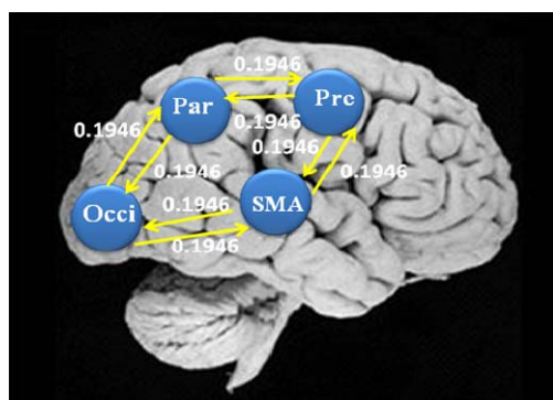
Fig. 4 The basic model without the visual stimulus
