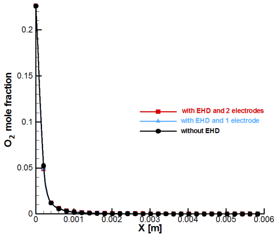
Fig. 11 [ O_2 ] mole fraction profile at h=5 \left(\frac{W}{m^2.K}\right)
