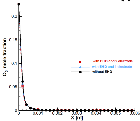
Fig. 12 [ O_2 ] mole fraction profile at h=10 \left(\frac{W}{m^2.K}\right)
