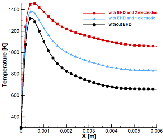
Fig. 7 Temperature profile at h=20 \left(\frac{W}{m^2.K}\right)
