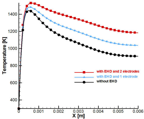
Fig. 6 Temperature profile at h=10 \left(\frac{W}{m^2.K}\right)
