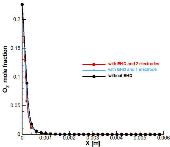
Fig. 13 [ O_2 ] mole fraction profile at h=20 \left(\frac{W}{m^2.K}\right)
