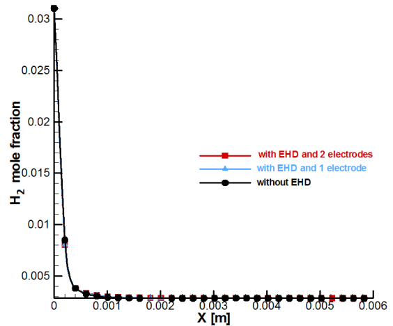
Fig. 14 [ H_2 ] mole fraction profile at h=5 \left(\frac{W}{m^2.K}\right)
