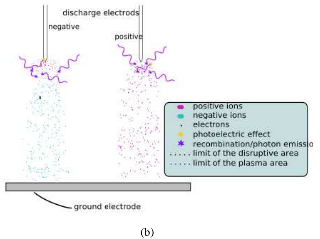
Fig. 2 (a) Electrical breakdown; (b) recombination and upkeep of the discharge [19]
