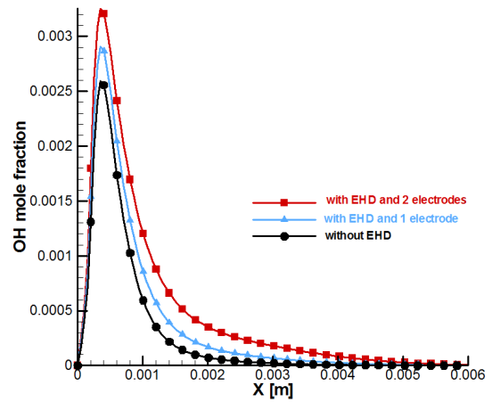
Fig. 9 [OH] mole fraction profile at h=10 \left(\frac{W}{m^2.K}\right)
