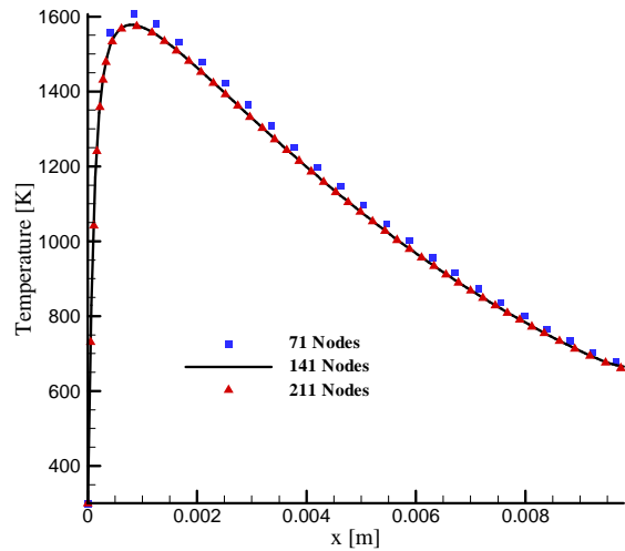
Fig. 4 Temperature profiles for different number of grids [21]
