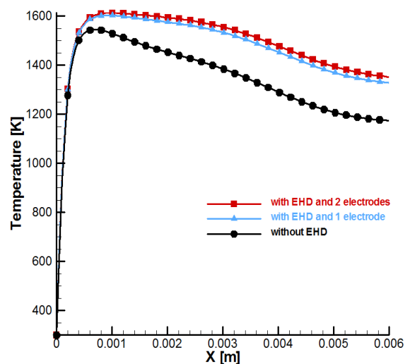
Fig. 5 Temperature profile at h=5 \left( \frac{\text{W}}{\text{m}^2.\text{K}} \right)
