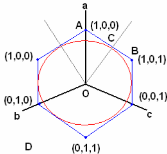
Fig. 4 Voltage vectors
