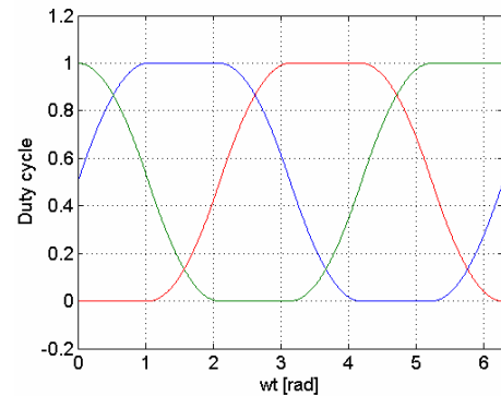
Fig. 3.a Flat-top PWM, 100% modulation depth
