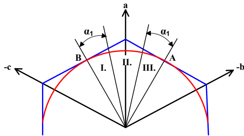
Fig. 5 Voltage vectors in DLF
