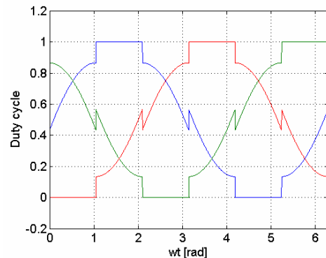
Fig. 3.b Flat-top PWM, 90% modulation depth
