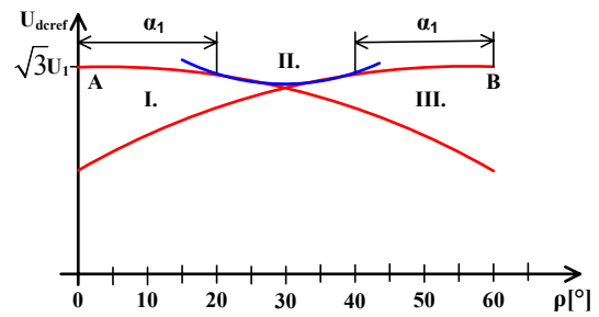
Fig. 6 DC voltage in the subsections
