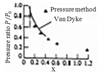
Fig. 13 Surface Pressure on Body Supporting a paraboloidal Shock; From Anderson [2] \gamma = 1.4 , M_o = \infty
