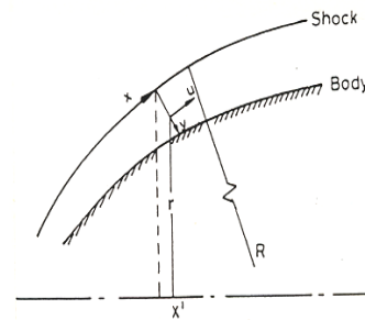
Fig. 3 Axisymmetric Geometry of Flow
