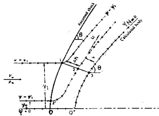
Fig. 2 2-Dimensional Geometry of Flow
