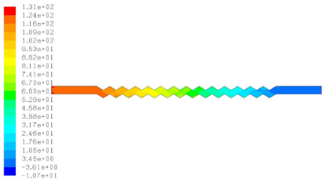
Fig. 16 Static pressure at Re 1400
