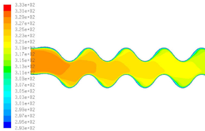
Fig. 43 Static temperature at the entrance part of the channel at Re 400
