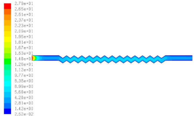
Fig.18 Turbulence intensity at Re 400
