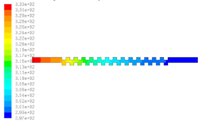
Fig. 51 Static temperature at Re 1400
