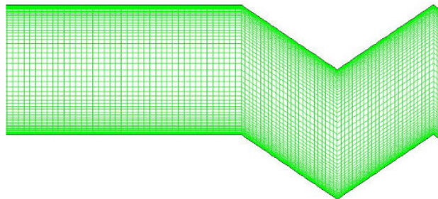
Fig. 8 Fine boundary layer grid
