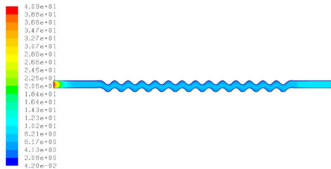
Fig. 40 Turbulence intensity at Re 1400
