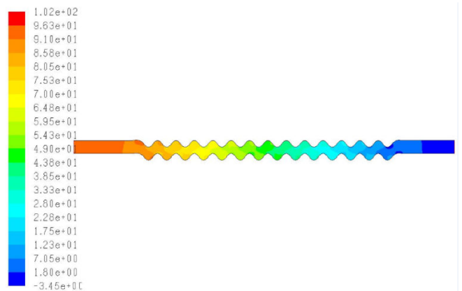
Fig. 38 Static pressure at Re 1400
