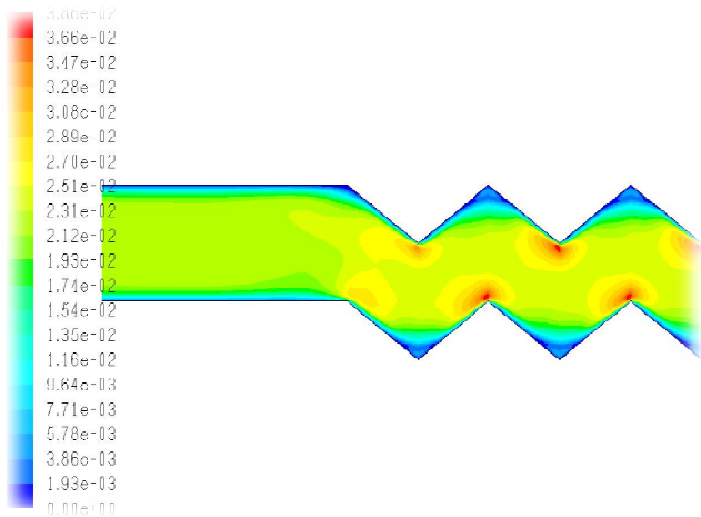
Fig. 11 Velocity magnitude at Re 400
