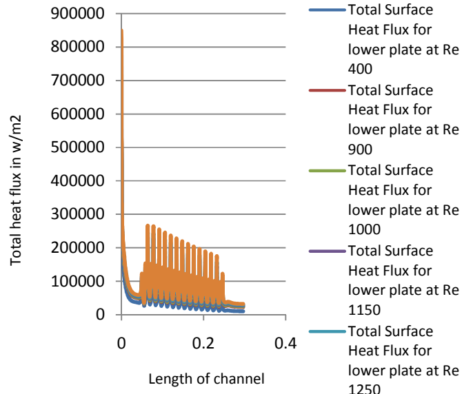
Fig. 27 Local total heat flux for triangular corrugated channel
