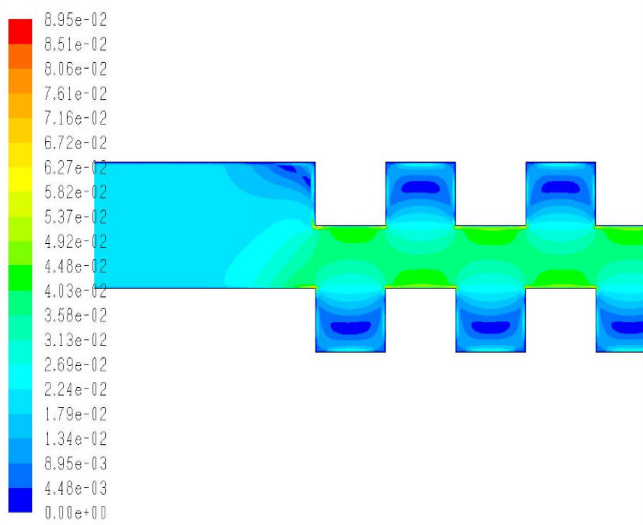
Fig. 44 Velocity magnitude at Re 400
