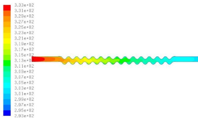
Fig. 41 Static temperature at Re 400
