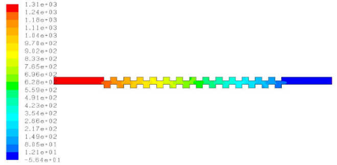
Fig. 46 Static pressure at Re 400
