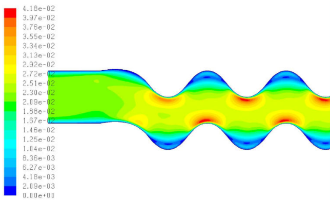
Fig. 35 Velocity magnitude at Re 400
