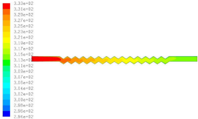
Fig. 25 Static temperature at Re 1400
