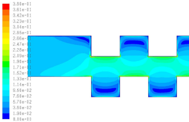
Fig. 45 Velocity magnitude at Re 1400
