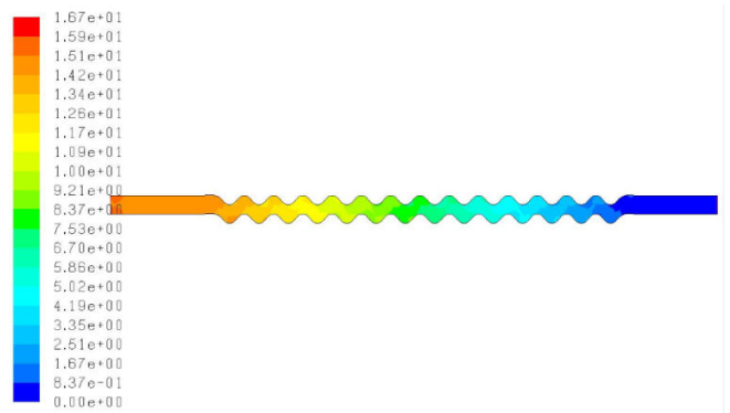
Fig. 37 Static pressure at Re 400
