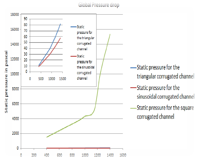
Fig. 53 Global pressure drop
