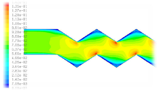
Fig. 12 Velocity magnitude at Re 1400
