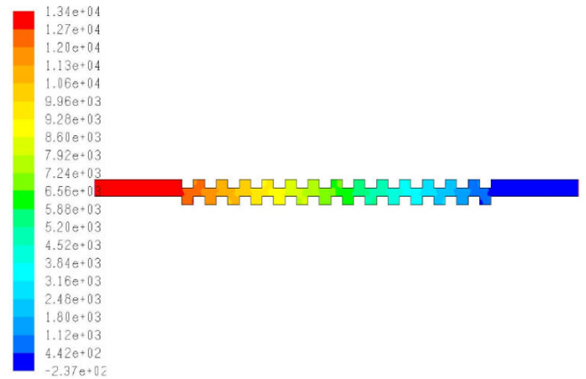
Fig. 47 Static pressure at Re 1400
