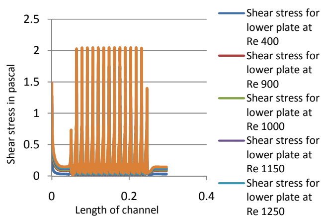
Fig. 21 Shear stress for one periodic corrugation
