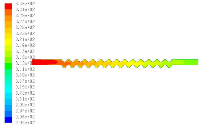
Fig. 42 Static temperature at Re 1400
