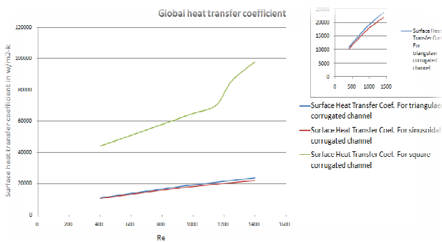
Fig. 58 Global heat transfer coefficient
