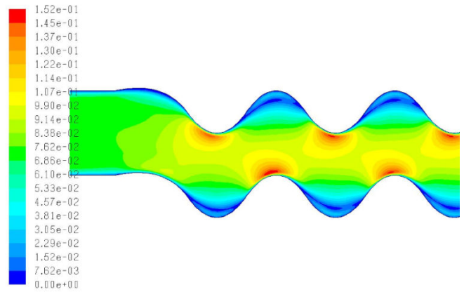
Fig. 36 Velocity magnitude at Re 1400
