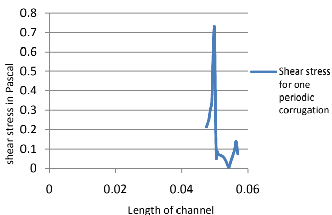
Fig. 20 Local shear stress for triangular corrugated channel
