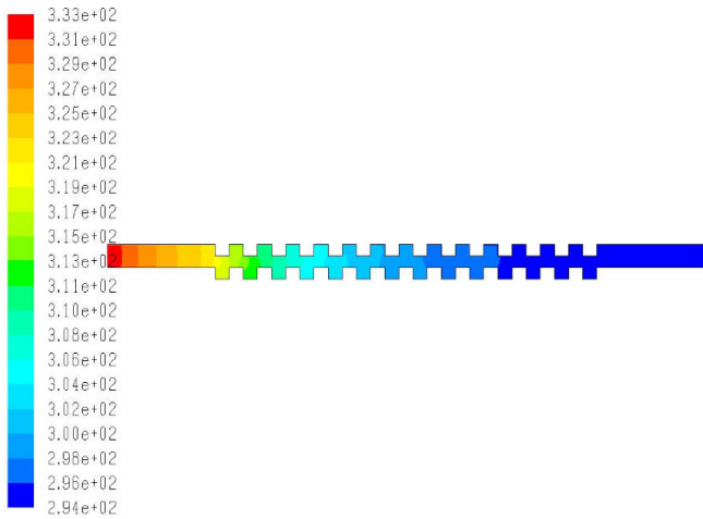
Fig. 50 Static temperature at Re 400
