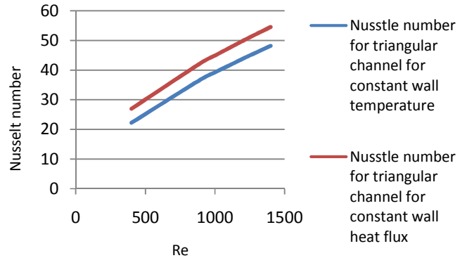
Fig. 59 Nusselt Number for triangular corrugated channel for two different boundary conditions
