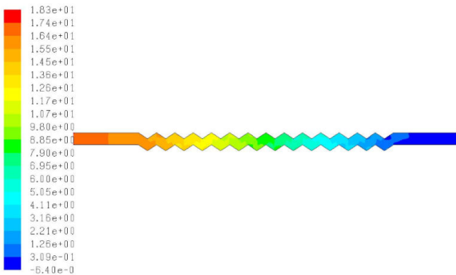
Fig. 15 Static pressure at Re 400
