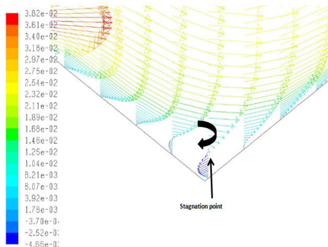
Fig. 31 Stagnation point
