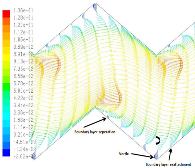
Fig. 14 Vector of velocity magnitude at Re 1400
