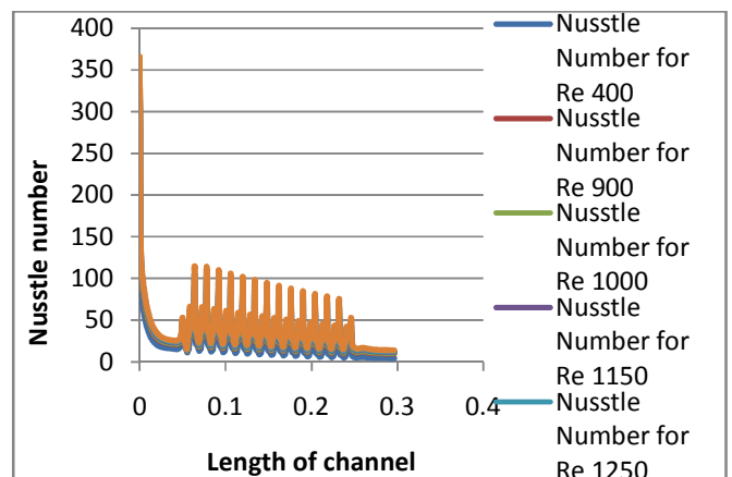
Fig. 29 Local Nusselt number for triangular corrugated channel
