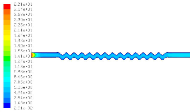
Fig. 39 Turbulence intensity at Re 400
