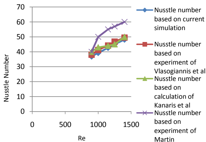
Fig. 33 Comparative plot between Nusselt number estimated by others and Nusselt number estimated by current estimation
