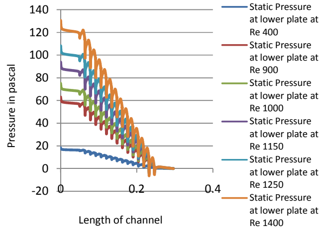
Fig. 17 Local pressure gradient for triangular corrugated channel
