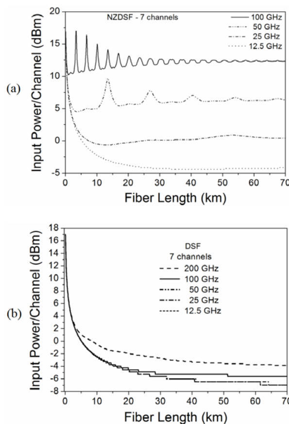
Fig. 6 Variation of the input power per channel as a function of the fiber length for a 7-channel system: (a) NZDSF, and (b) DSF fibers.
