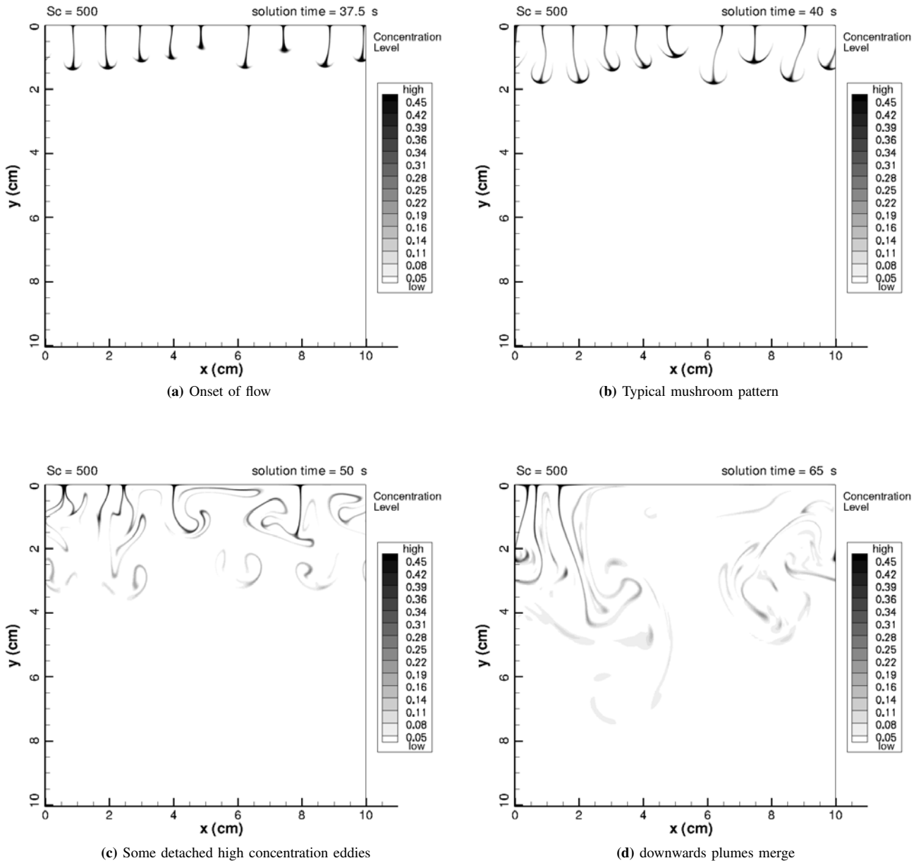
Fig. 2: A sequence of oxygen concentration contour maps visualizing the onset of the Rayleigh-Bénard instability subsequent mixing. 800 \times 300 gridpoints. The surface temperature T_S = 17^\circ\text{C} . The bulk temperature T_0 = 20^\circ\text{C}
