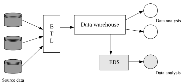
Fig. 3 Solution architecture
