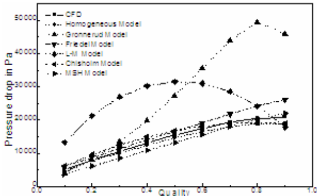
Fig. 11 Pressure drop of R134a at 40°C with G= 1058 \text{ kg/m}^2\text{s}
