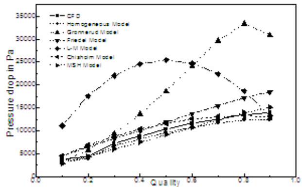
Fig. 12 Pressure drop of R407C at 40°C with G= 1058 \text{ kg/m}^2\text{s}
