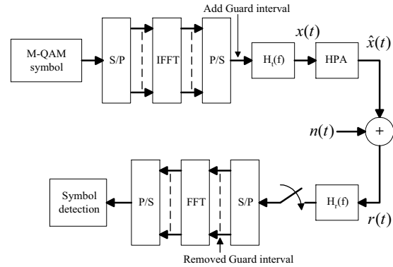
Figure 1. Baseband OFDM system.
