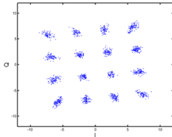
Figure 2. The received signal constellation for a 16-QAM OFDM using TWTA with OBO=7 dB and N=128 subcarriers.
