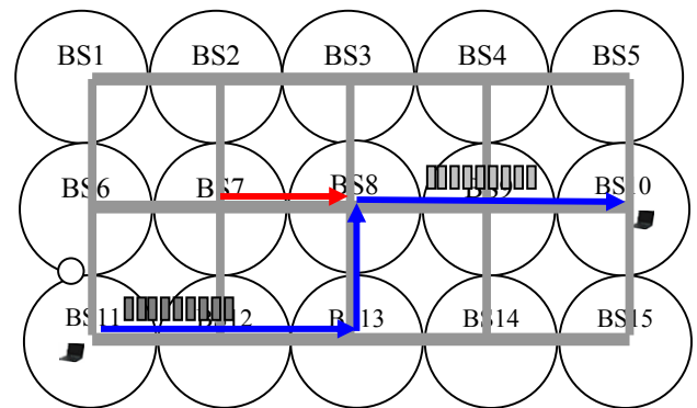
Fig. 2 Bandwidth Allocation to ABR mobile node when the node handover to another cell
