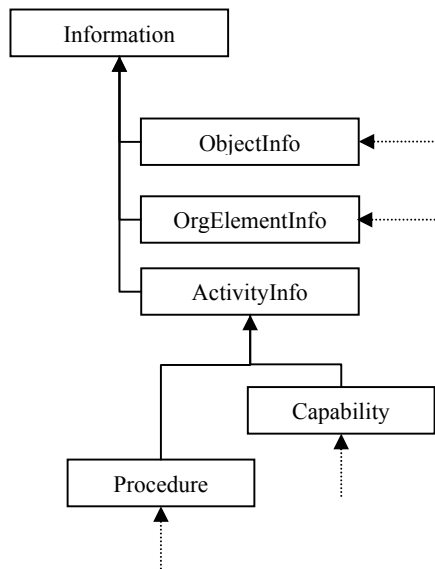
Fig. 4 Ontology fragment at the Generic Level
