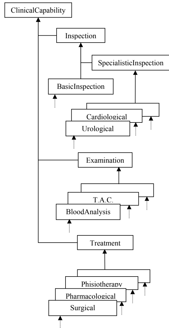
Fig. 5 Ontology fragment at the Partial Level
