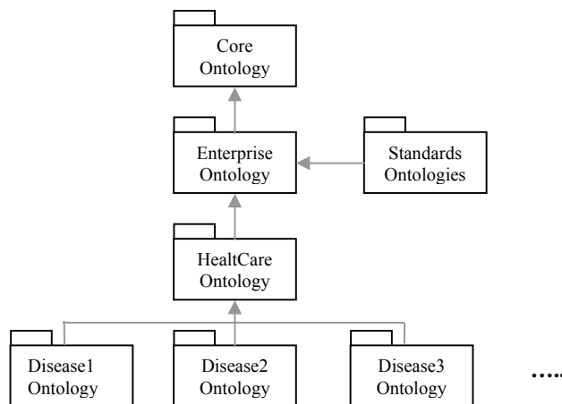
Fig. 2 Paradigma Reference Ontology Levels
