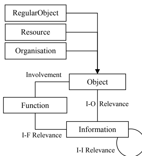
Fig. 2 Paradigma Reference Ontology Levels
