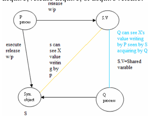
Fig. 4. Operation with processes
