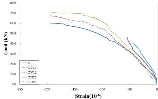
Fig. 16 Strain Curve C7
