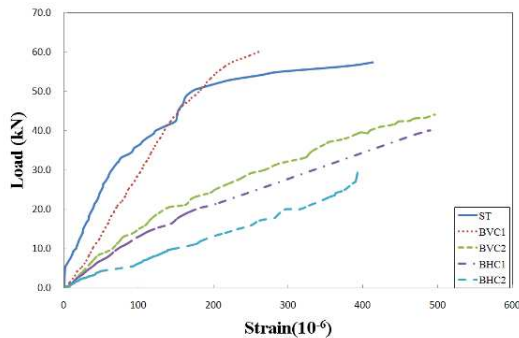
Fig. 15 Strain Curve C3
