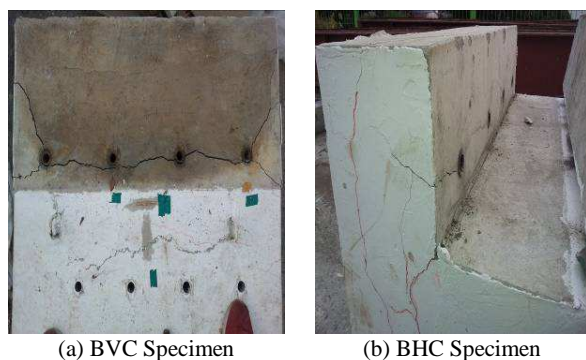
Fig. 18 Crack pattern of Interface
