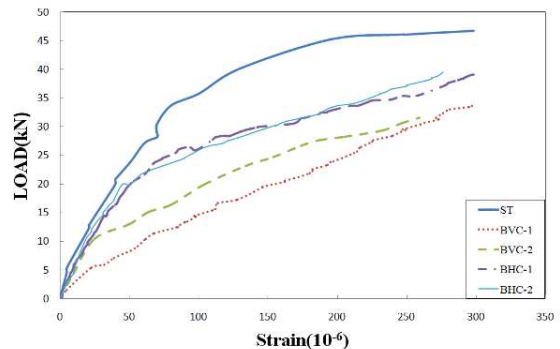
Fig. 13 Strain Curve S1
