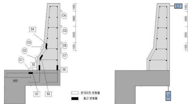
Fig. 9 Location of Strain Gauges
