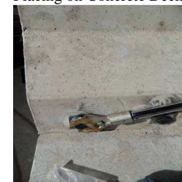
4. Connecting Barrier to the Deck
