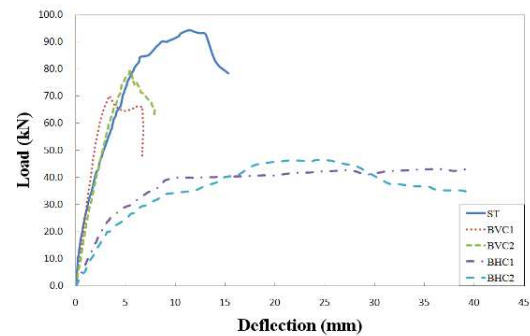
Fig. 12 Load-Deflection Curve at LVDT2
