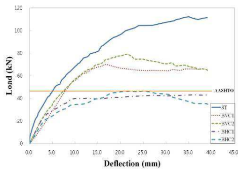
Fig. 11 Load-Deflection Curve at LVDT1
