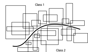
Fig. 2 Fuzzy min-max hyperboxes along the boundary
