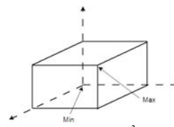
Fig. 1 Hyperbox in R^3 defined from its min and max points
