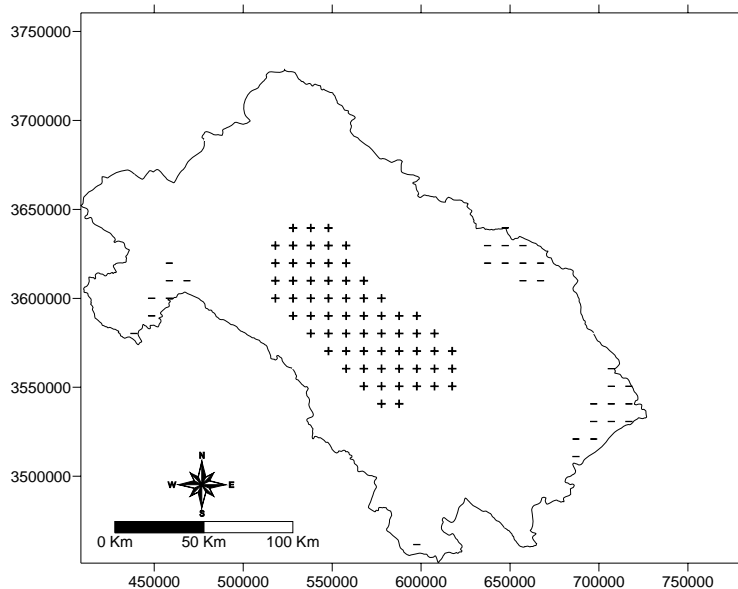
Fig.6 Temperature changes in Zayanderood watershed
