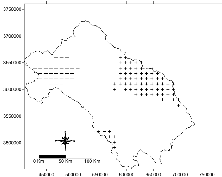
Fig.4 Precipitation changes in Zayanderood watershed
