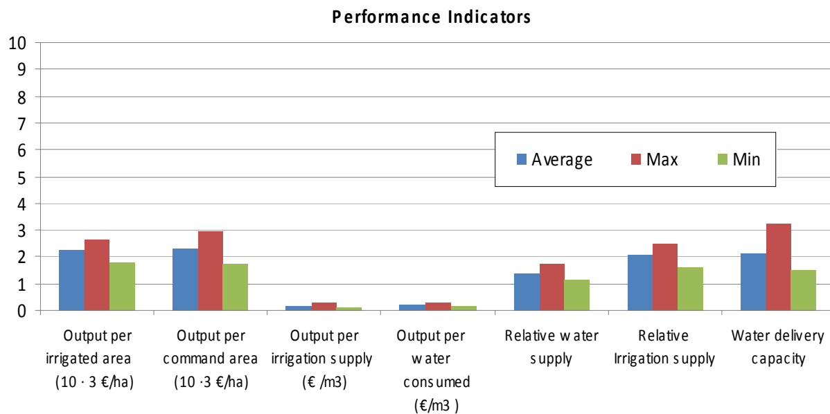
Fig. 4. Performance indicators of Axios River irrigations systems
