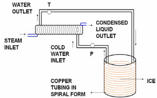
Fig. 3 Condensation setup
