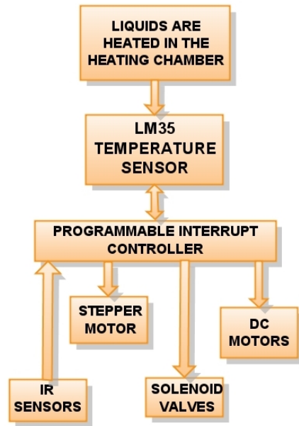
Fig. 1 System block diagram
