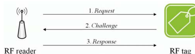
Fig. 2 serverless based RFID system
