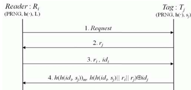
Fig. 3 Authentication protocol proposed by Tan et al.
