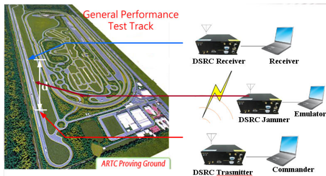
Fig. 1 System operation Testbed
